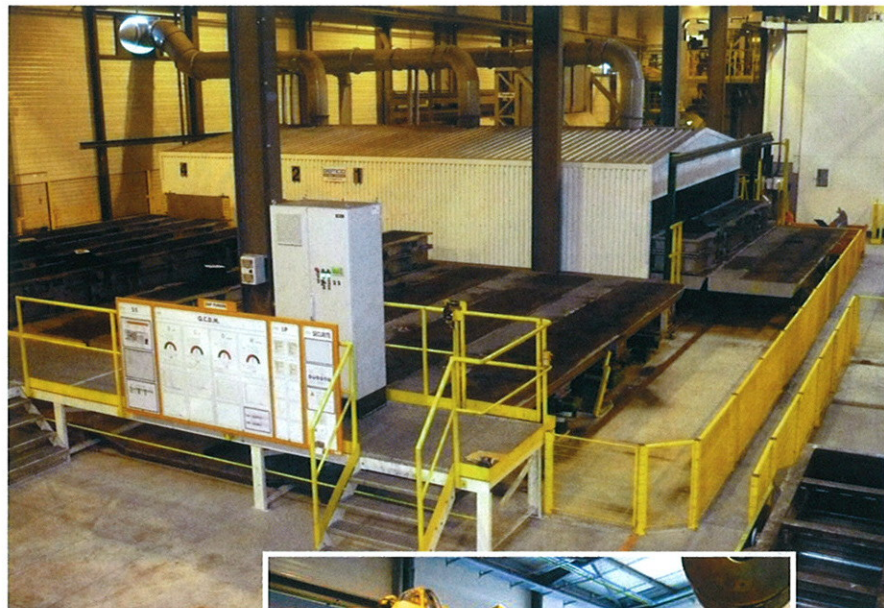
Above: Pouring and cooling line
